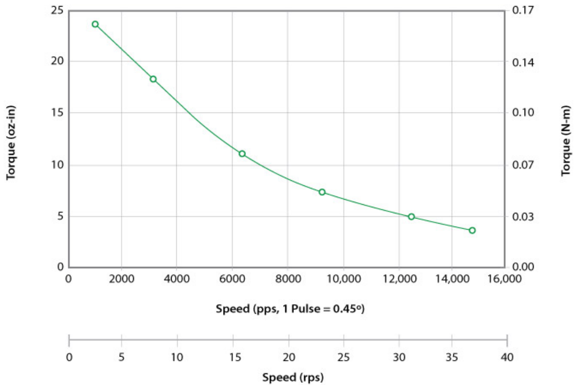
Z417-17-04 (0.9° Step Motor) 24VDC, 0.7 Amp Peak, Bipolar, 1/2 Stepping
